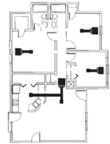
Fujitsu Quad Zone Concealed Ceiling System
